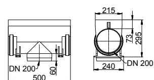
Vertical outlet - Nominal width 200 mm
