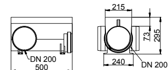
Outlet left/right - Nominal width 200 mm
