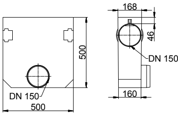
Nominal width 150 mm
