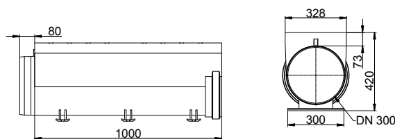
Nominal width 300 mm
