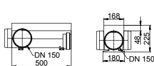
Outlet left/right - Nominal width 150 mm
