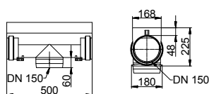
Vertical outlet - Nominal width 150 mm
