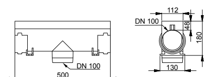
Vertical outlet - Nominal width 100 mm
