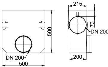
Nominal width 200 mm
