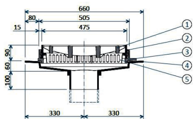
① grate with hinge ② frame ③ pot ④ plate ⑤ dirt basket
