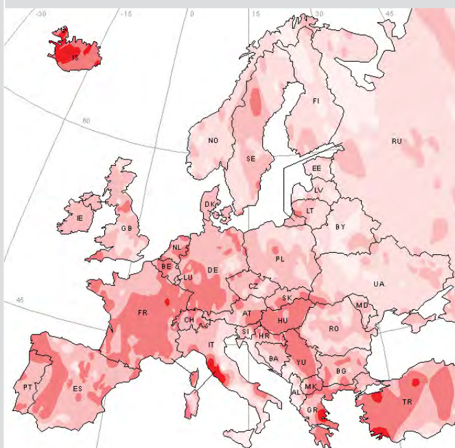
Geothermal Heat-Flow Density
