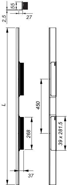
shower channel CeraWall Select Duo satin stainless steel
