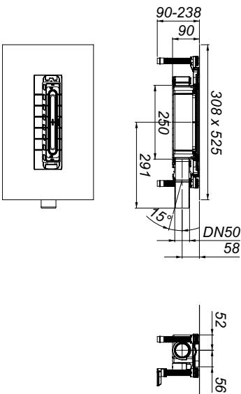
drain body DallFlex 2.0
