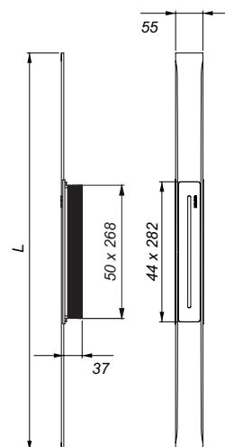
shower channel CeraFloor Select polished stainless steel
