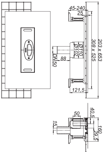
drain body CeraFlex vertical
