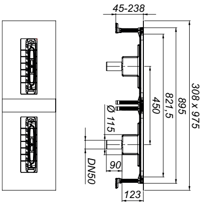
drain body DallFlex 2.0 Duo vertical
