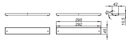
cover plate CeraWall Individual Duo
