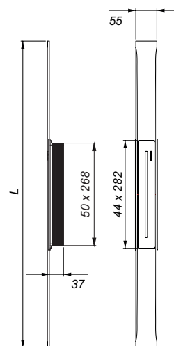
shower channel CeraFloor Select satin stainless steel
