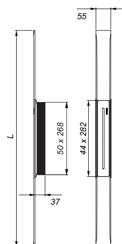
shower channel CeraFloor Select red gold matt
