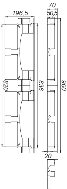
sound-insulating element DallFlex Duo Plan
