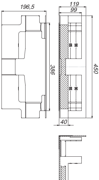
sound-insulating element DallFlex 115
