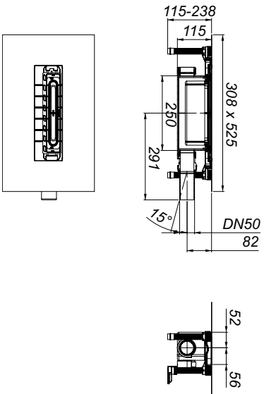
drain body DallFlex 2.0 115
