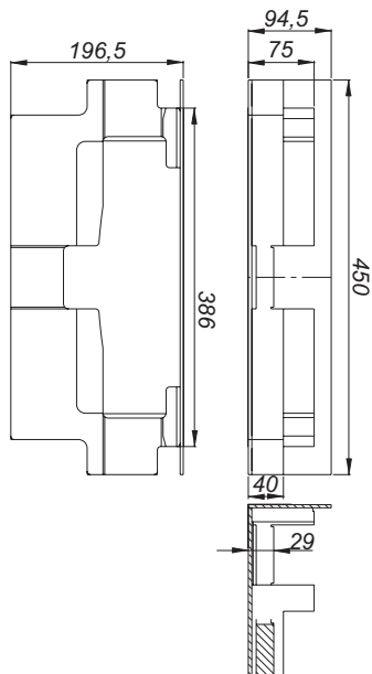
sound-insulating element DallFlex/CeraFlex
