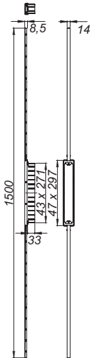
shower channel CeraFloor Individual black matt
