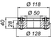
Fire protection element DN 50
