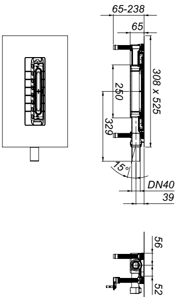
drain body DallFlex 2.0 Plan
