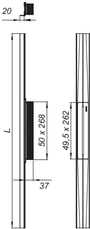
shower channel CeraWall Pure
