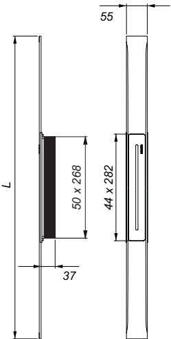
shower channel CeraFloor Select brass matt
