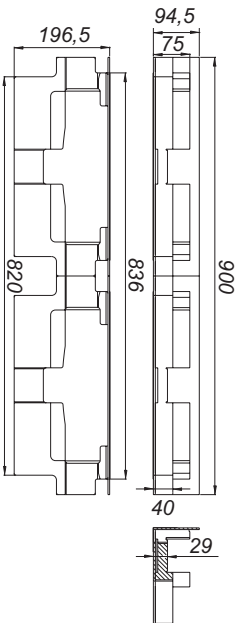
sound-insulating element DallFlex Duo
