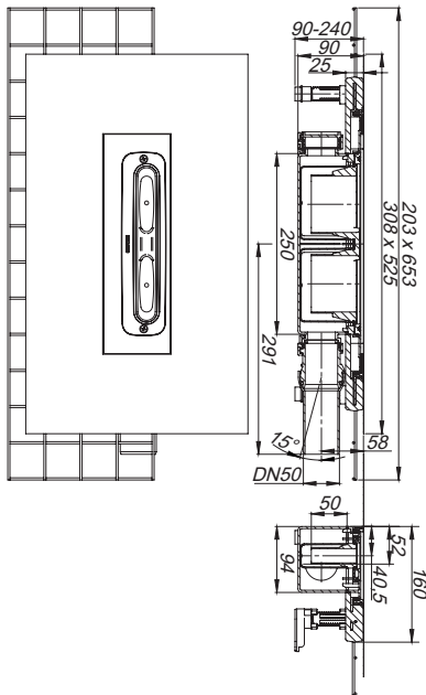
drain body CeraFlex
