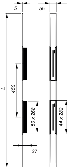
shower channel CeraFloor Select Duo satin stainless steel
