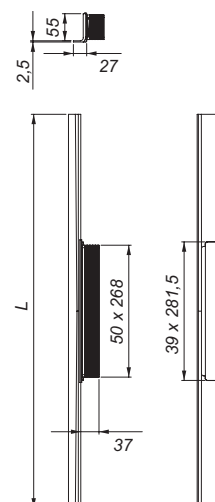
shower channel CeraWall Select satin stainless steel
