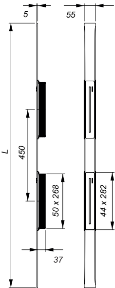
shower channel CeraFloor Select Duo black matt
