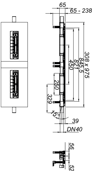
drain body DallFlex 2.0 Duo Plan
