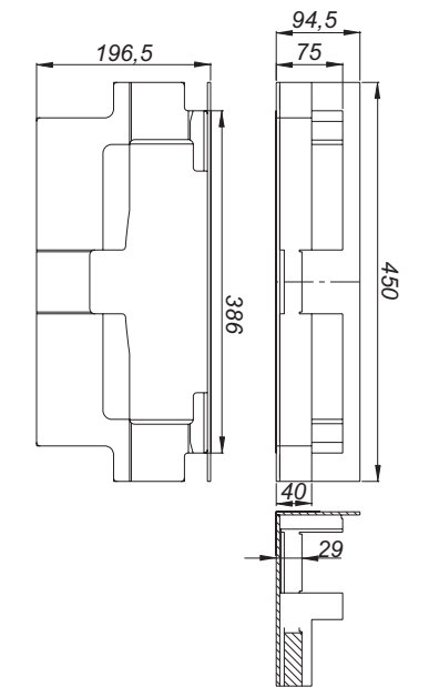
sound-insulating element DallFlex/CeraFlex
