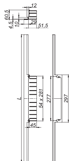
shower channel CeraWall Individual black matt
