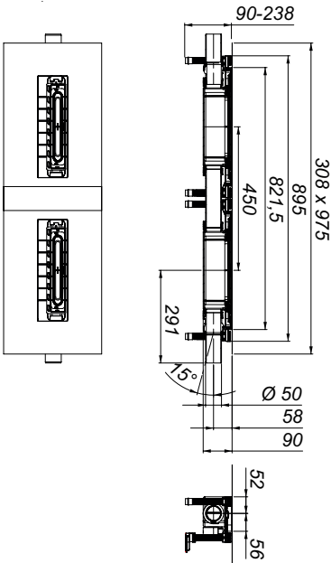
drain body DallFlex 2.0 Duo
