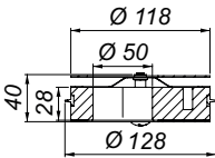
Fire protection element DN 50.1
