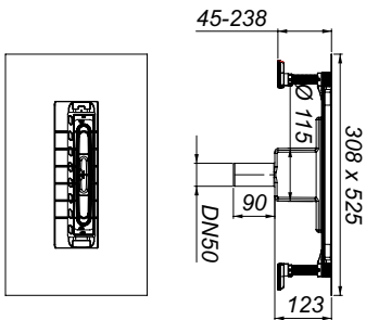
drain body DallFlex 2.0 vertical
