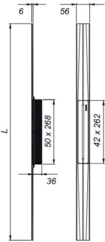
shower channel CeraFloor Pure
