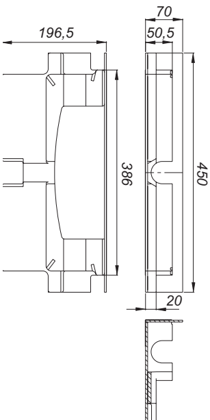
sound-insulating element DallFlex/CeraFlex Plan
