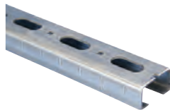
C-Channel Type E2L, Perforated
