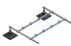
Pyramid H-Frame Post Base
