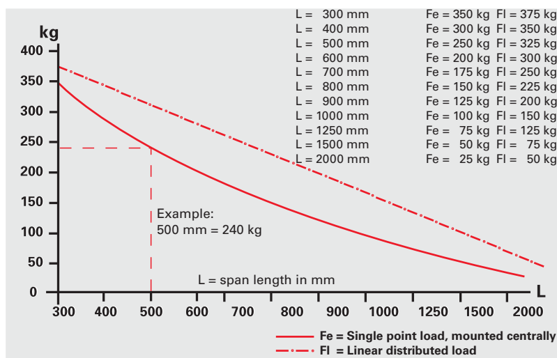
Load Chart for L = 300 mm - 2000 mm
