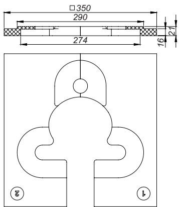
mounting aid DalIDrain Plan
