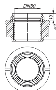
bathtub connector DallDrain
