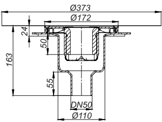
drain body DalIDrain vertical
