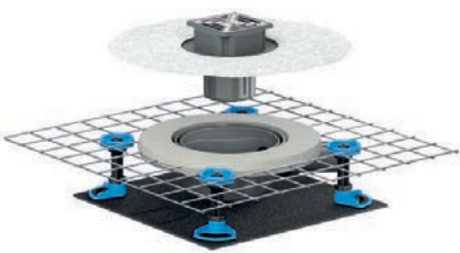
sound-insulating floor drain CeraDrain Pure, 100 x 100 mm
