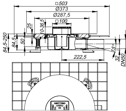
floor drain CeraDrain Select, 100 x 100 mm
