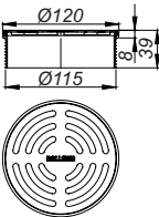
grating DalIDrain Select, d: 120 mm
