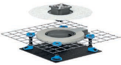
sound-insulating floor drain CeraDrain Select Plan, 100 x 100 mm
