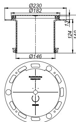
raising piece DalIDrain
