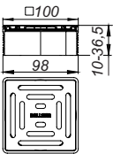
grating DalIDrain Select, 100 x 100 mm
