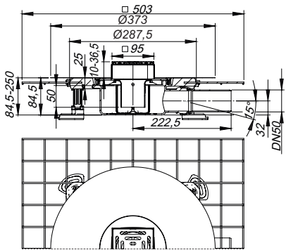
floor drain CeraDrain Pure 100 x 100 mm
