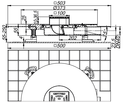
sound-insulating floor drain CeraDrain Select Plan, 100 x 100 mm
