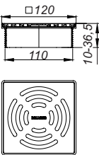
grating DalIDrain Select, 120 x 120 mm
