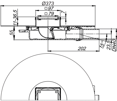
floor drain DalIDrain Individual Plan OM
