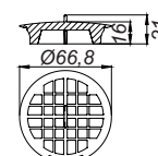
hair sieve DallDrain
