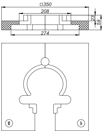
mounting aid DalIDrain
