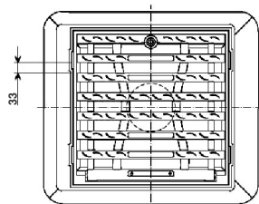
① grate with hinge ② frame ③ pot ④ plate ⑤ dirt basket
